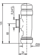
Toilet flush button 3/4" G. thread plug cock intel. Outlet for 26x28 pipe. Flow 1.5 l/min.
