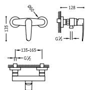
Single lever shower mixer Anti-limescale hand shower with directable support. Shower hose satin.
