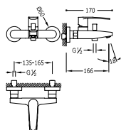
Single lever bath and shower mixer Anti-limescale hand shower with directable support. Shower hose satin.
