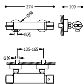
Wall thermostatic shower mixer (Anti-limescale hand shower with directable support. Shower hose satin).
